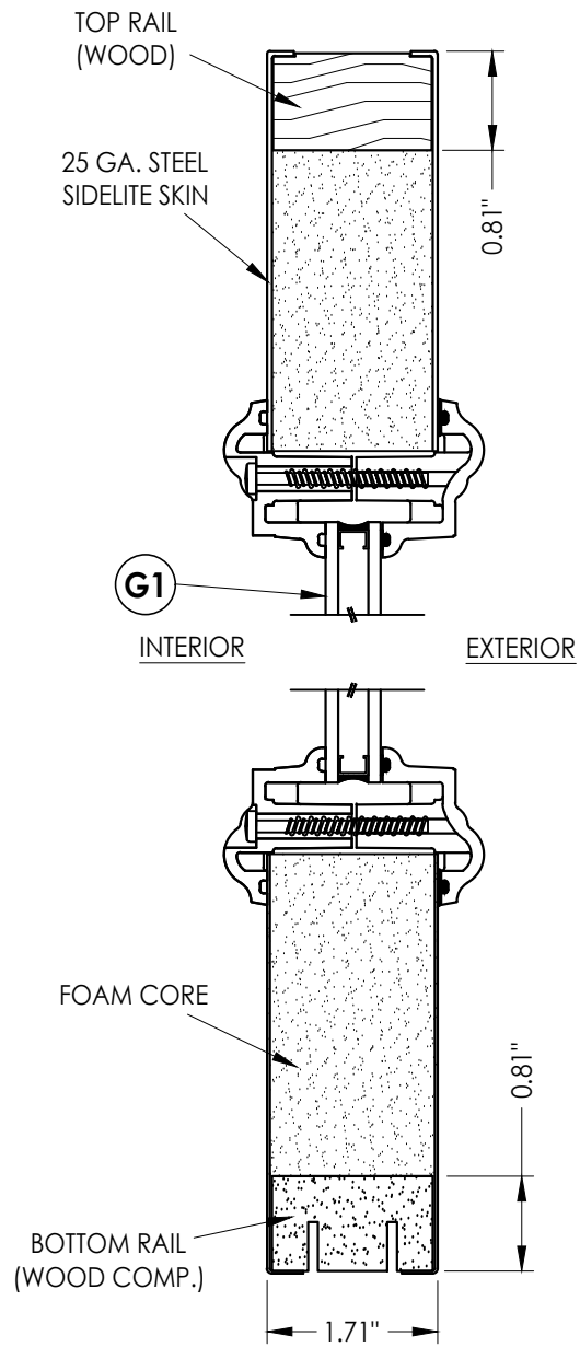
2 4 VERTICAL CROSS SECTION
