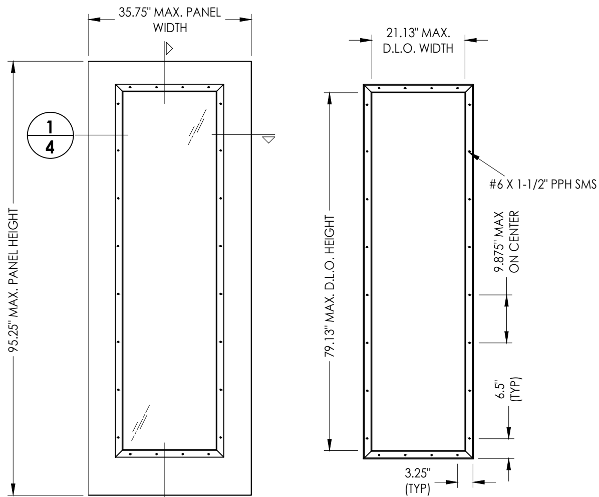
2 4 SIDELITE PANEL Masonite Steel (Wood Edge)
