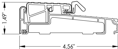
T11 OUTSWING THRESHOLD ZOB4565
