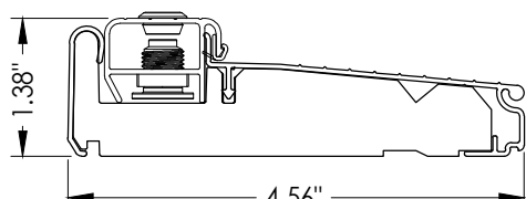
T4 INSWING ADJUSTABLE THRESHOLD ZAIAA4565FN
