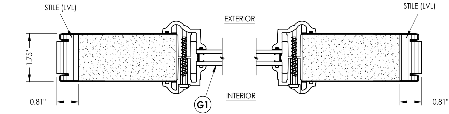
1 4 HORIZONTAL CROSS SECTION
